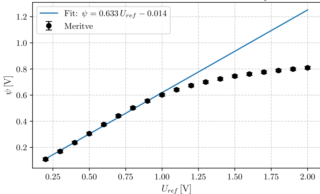
Measured \psi vs Reference Voltage U_{ref}
